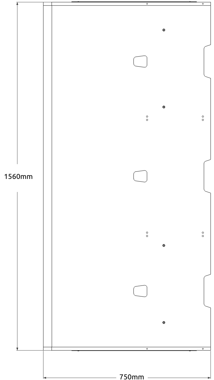
TOP VIEW
