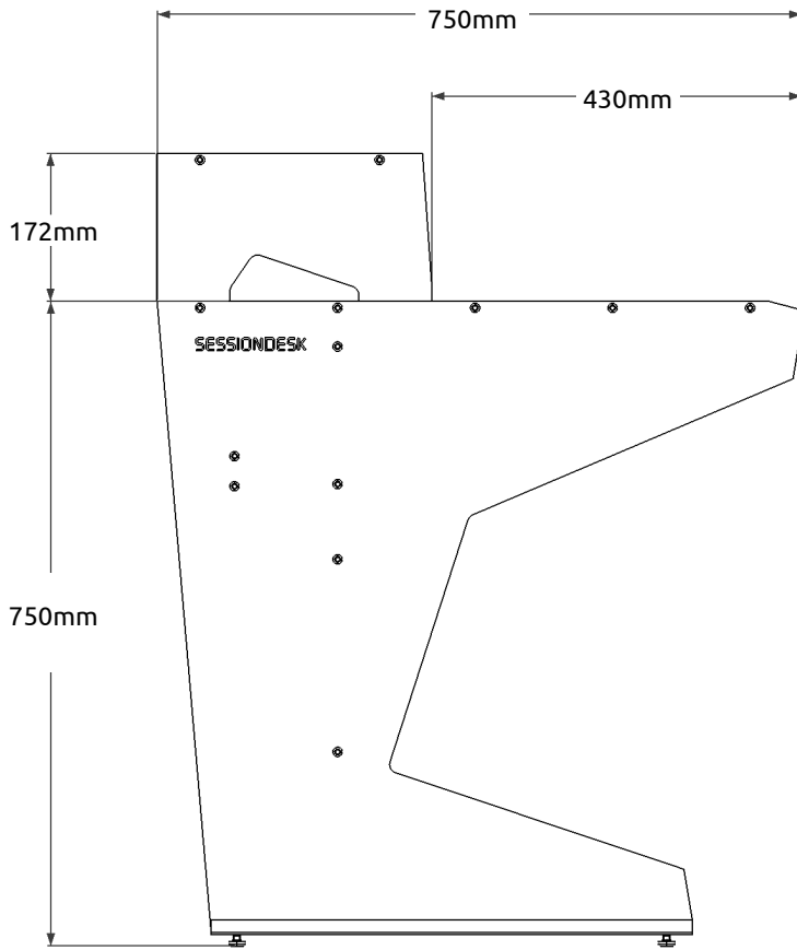
SIDE VIEW
